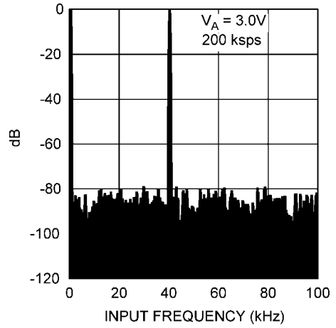
Spectral Response - 3V, 200 ksp/s
