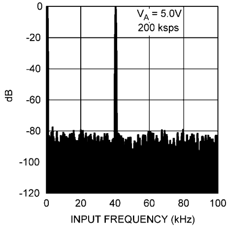
Spectral Response - 5V, 200 ksp/s
